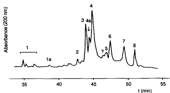
Fig. 5. Comparative profile of collagen type-I CNBr peptides run in a surface untreated capillary but with the addition of 7.5% acetonitrile to the run buffer. Identification of peptides same as in Fig. 1, except for \alpha_1\text{CB}_4 (1a) and \alpha_1\text{CB}_7 (4a).
