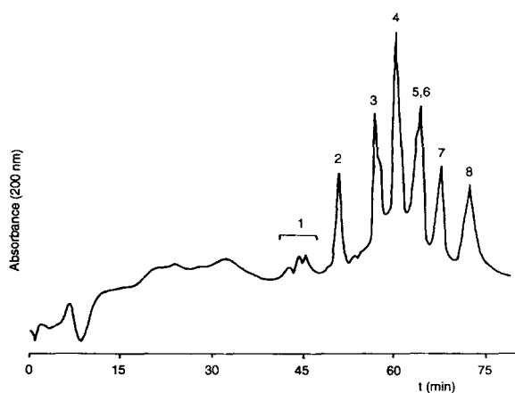
Fig. 2. Reversed-phase HPLC of type-I collagen CNBr peptides (300 \mu\text{g} ). Linear gradient from 12.8 to 44.8% (v/v) acetonitrile in water, mobile phase made 10 mM with respect to HFBA; flow-rate, 1.0 ml/min. Peak identification as in Fig. 1.
